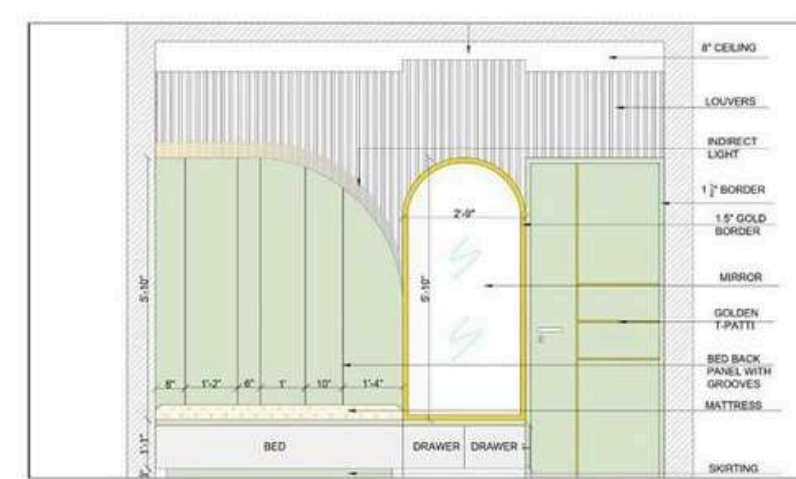
Detail 2D Drawings
